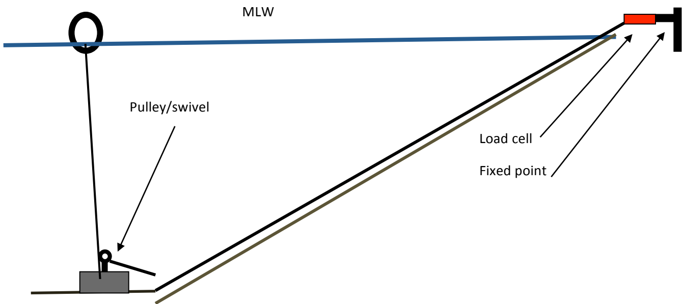
Figure 2-4. Schematic of mooring/taut line system indicating load cell placement at the fixed point.
