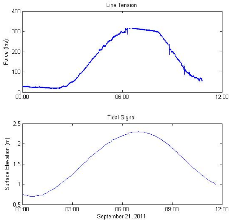
Figure 2-5. Measured line tension is shown in the top plot and the corresponding tide signal is shown in the bottom plot. The maximum tension was 325 lbs.
